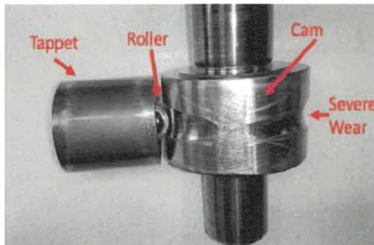
Figure 8: Effects of the Rotation of the Roller
