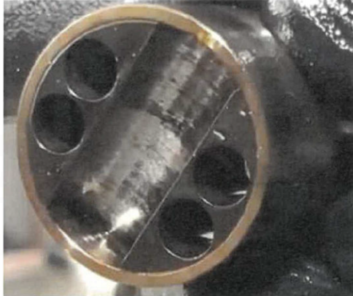
Figure 7: Wear on the Diamond Coating
