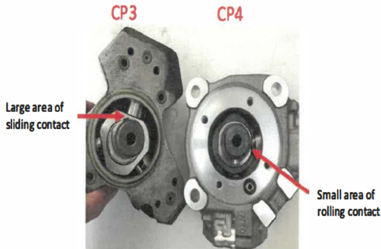
Figure 3: Comparison of CP3 and CP4 fuel pumps
