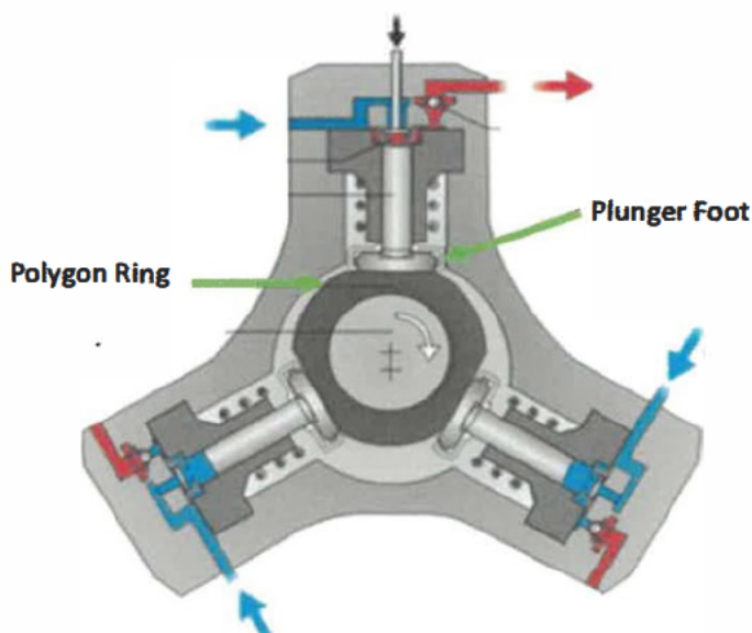
Figure 1: CP3 Fuel Pump
